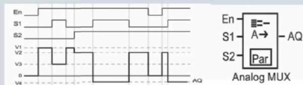
Analog-MUX
