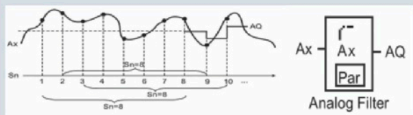
Analogfilter
